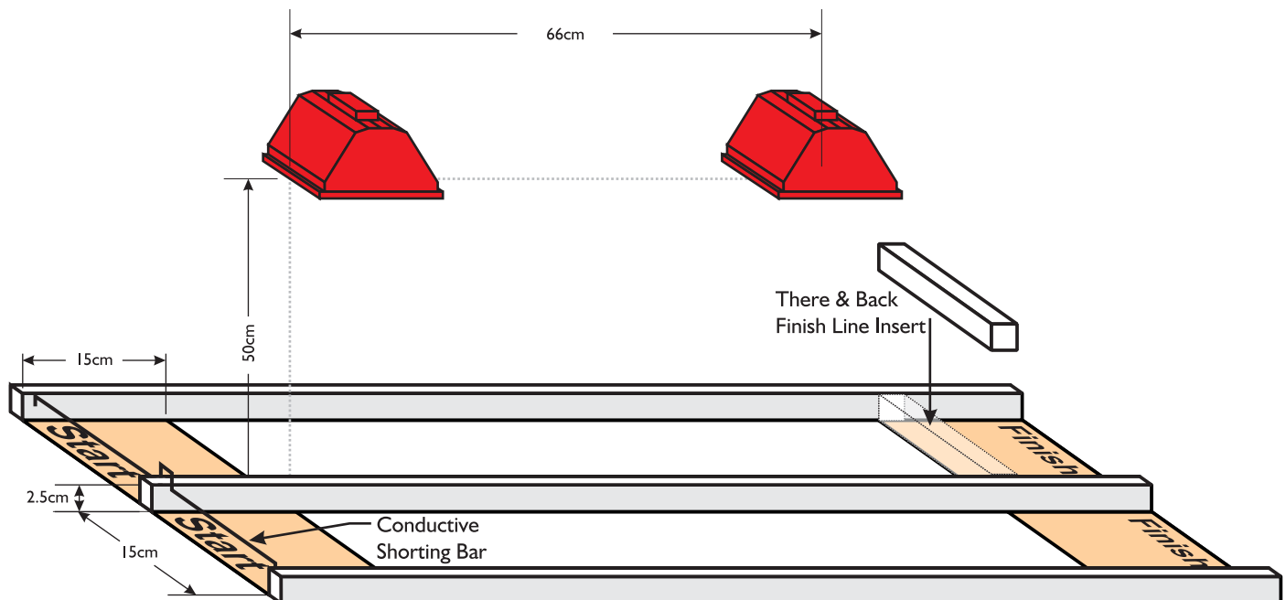
The Solaroller platform
